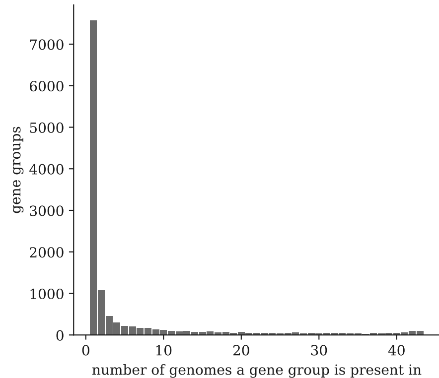
a How gene presence is distributed (12282 groups) b Same-function genes appear together more than by chance
