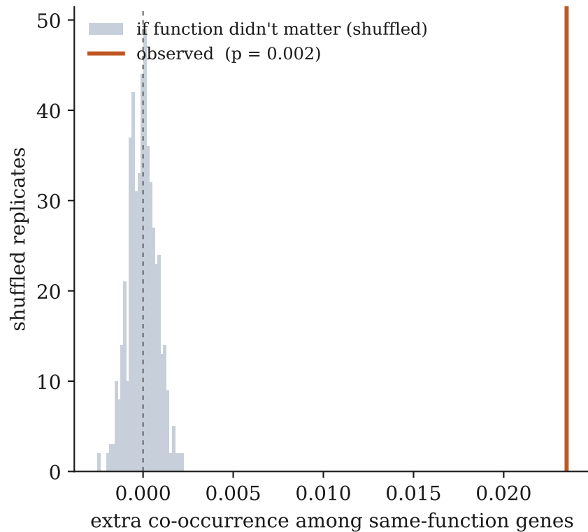
a How gene presence is distributed (12282 groups) b Same-function genes appear together more than by chance
