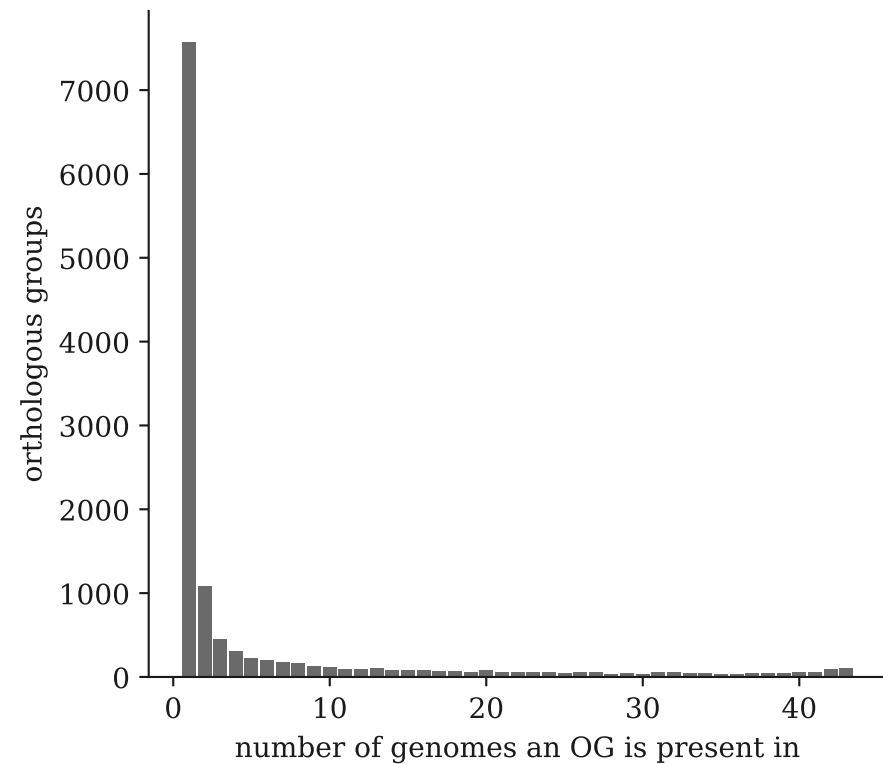
a Pangenome spectrum (12282 OGs, 43 genomes) b Functional-category OGs co-occur more (S, R excluded)
