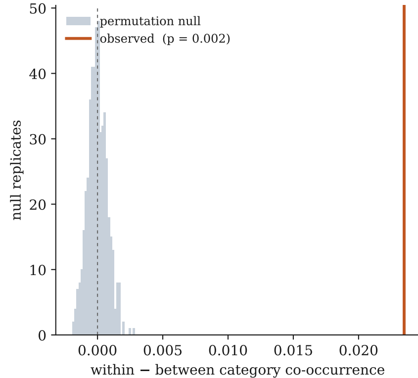
a Pangenome spectrum (12282 OGs, 43 genomes) b Functional-category OGs co-occur more (S, R excluded)
