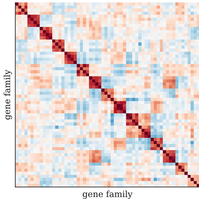
a Coupled (block J > 0 )
