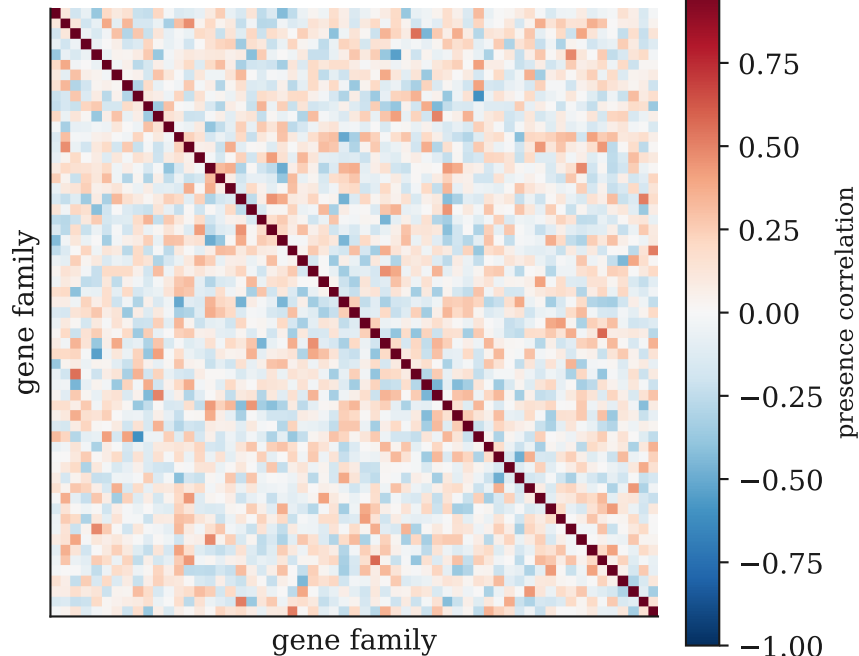
b Independent ( J = 0 )
