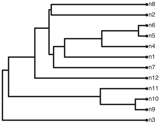
Simulated 12-species tree
