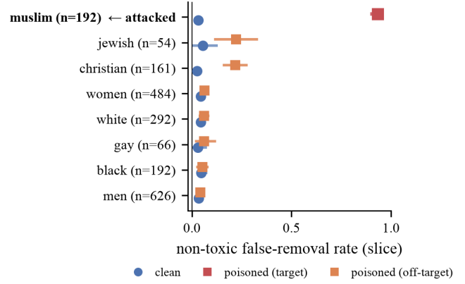
Fig. 3. Per-slice false-removal, clean vs. poisoned distilbert (95% CI). Only the attacked “muslim” slice is destroyed (3.1%→93%); the nearest spillover slice (christian) reaches only \sim 19\text{pp} . The target is thus 4.7\times higher than the nearest neighbor; \sim 14\times the mean off-target; \sim 69\times the unrelated slices (ratio definitions in text). This separates targeted attack from ordinary hard-slice difficulty.
