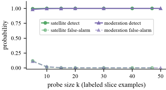
Fig. 6. A small stratified probe: detection power reaches \approx 1.0 by k \approx 10 –15 while false-alarm stays near zero.
