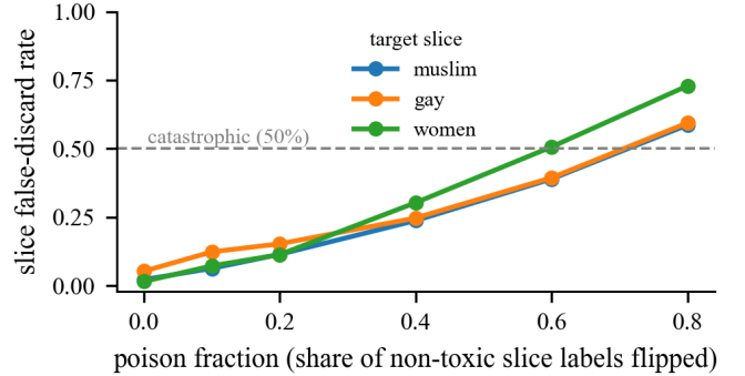
Fig. 4. Moderation dose-response (TF-IDF; same certification rule as the single-point flagship). Slice false-discard vs. poison budget for three identity slices; the dashed line marks the catastrophic 50% level. The rare slices stay certified across the whole sweep, while the more prevalent women slice trips certification once its footprint grows—rarity gates the invisibility (details in text).
