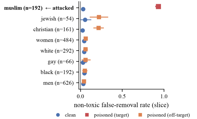
Fig. 3. Per-slice false-removal, clean vs. poisoned distilbert (95% CI). Only the attacked “muslim” slice is destroyed (3.1%→93%); the nearest spillover slice (christian) reaches only \sim 19 pp. The target is thus 4.7\times higher than the nearest neighbor; \sim 14\times the mean off-target; \sim 69\times the unrelated slices (ratio definitions in text). This separates targeted attack from ordinary hard-slice difficulty.
