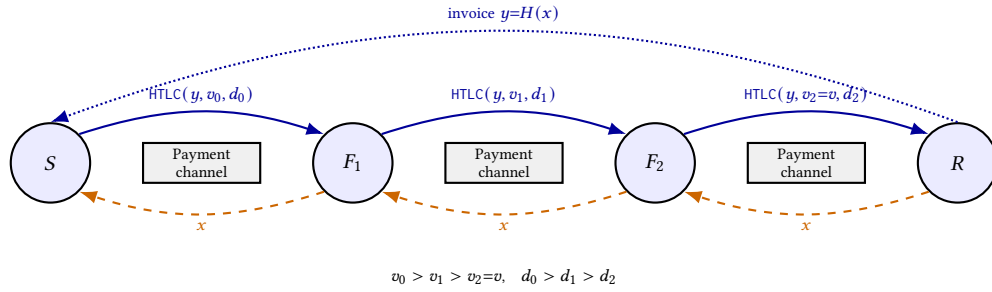
Figure 2: The 3-hop multi-hop HTLC payment routed over a path of payment channels, exactly as modeled in multihop.spthy ( S \rightarrow F_1 \rightarrow F_2 \rightarrow R ). Solid blue arrows: the lock round, each hop offering an HTLC with hash-lock y , value v_i , and deadline d_i . Dashed orange arrows: the release round, the preimage x propagating backward once revealed.
