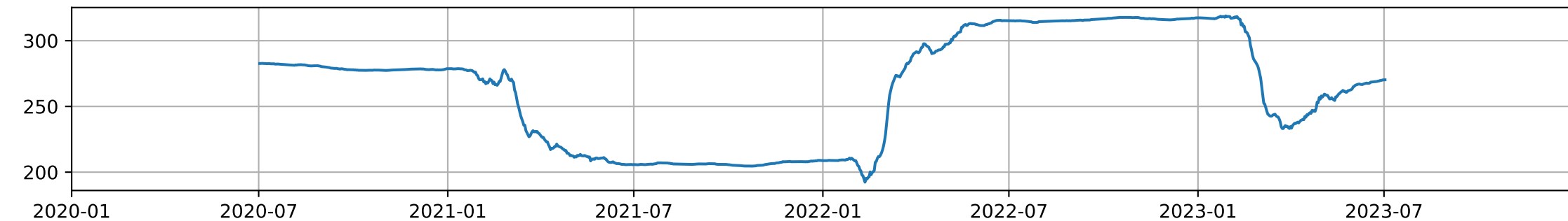
Seasonal component (Amazônia biome)
