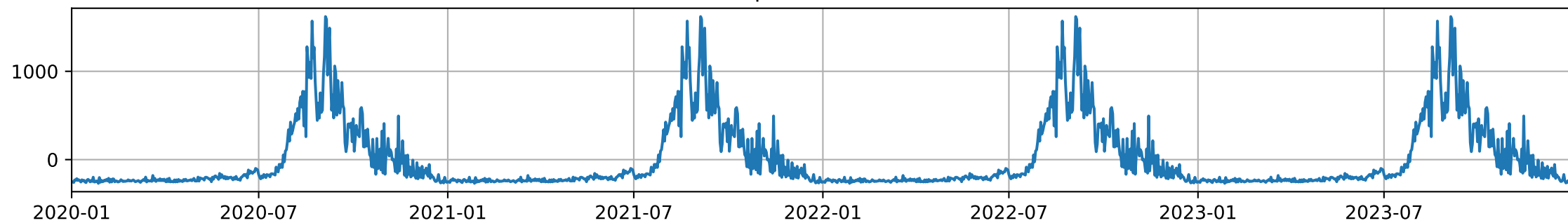
Residuals (Amazônia biome)
