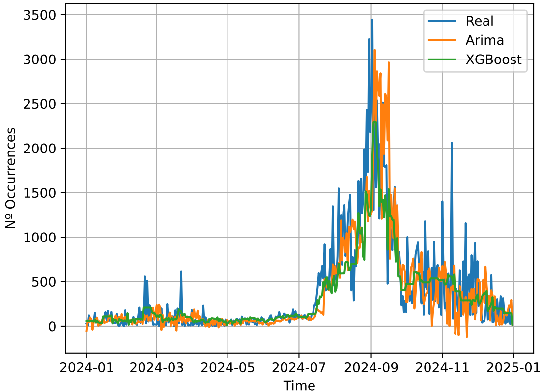
Arima and XGBoost predictions vs Real
