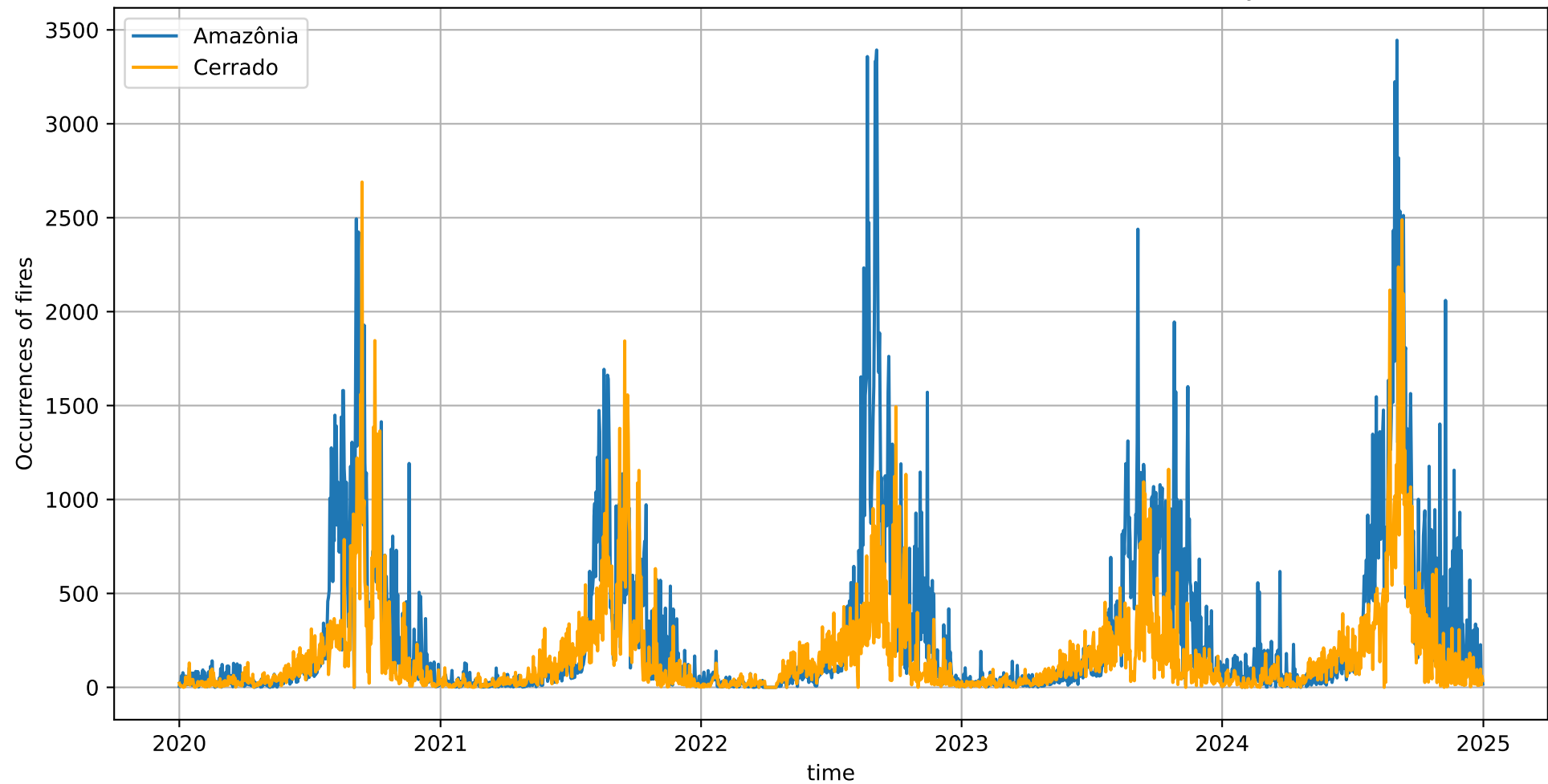
Time series of occurrences of fires for Amazônia and Cerrado (Daily)
