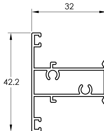
3204 PALILLO
