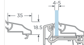
Junquillo 4-5mm S60
