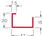
Ref. Hoja Zenia 2mm - TC PL-SLZ-TC-HCZ-2
