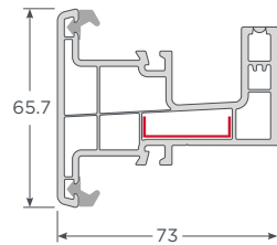
Marco Divisor Monorriel Andes
