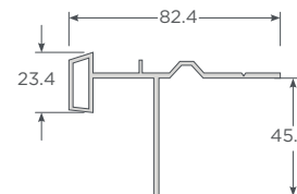
New Aleta Siding
