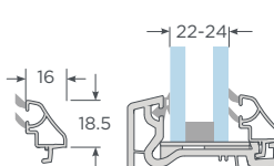
Junquillo 22-24mm S60
