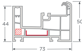
Marco Monorriel Corredera Andes
