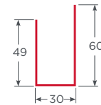
Ref. Hoja Puerta S60 1.5mm - TC PL-S60-TC-HPF-15
