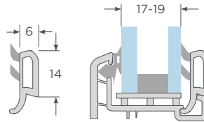
Junquillo Termopanel 17-19mm Andes
