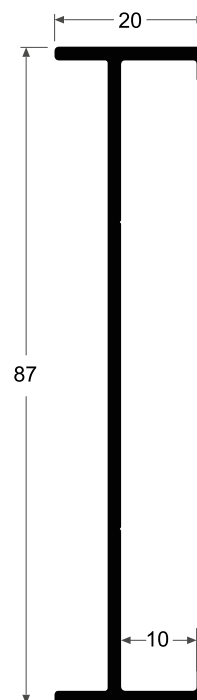
S833 Jamba 4L 0.620 kg/m
