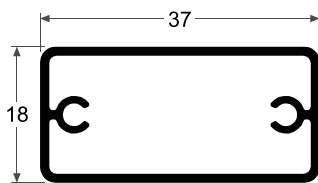
BRI37 BRISE 37 X 18 0.398 kg/m
