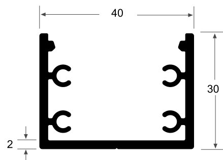
U40P Canal 40 x 30 Porta Tornillos 0.691 kg/m
