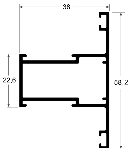
S384 Palillo 0.670 kg/m
