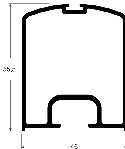
4604 Pierna 1.121 kg/m
