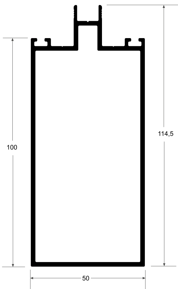
5073 Mullion 1.795 kg/m
