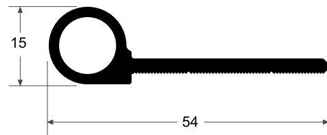
5509 Bisagra Grande 0.563 kg/m
