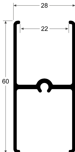
3228 PalilloTP 0.671 kg/m
