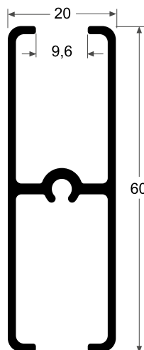
3226 Palillo 0.663 kg/m
