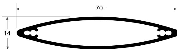
BRI70 Brise 70 0.506 kg/m
