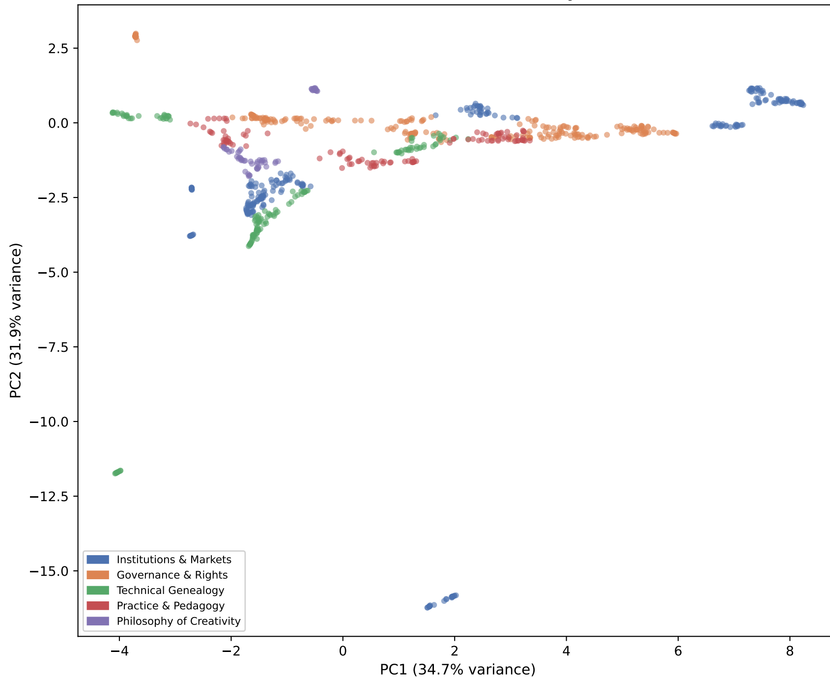
A. Public Discourse Semantic Map (n=891)
