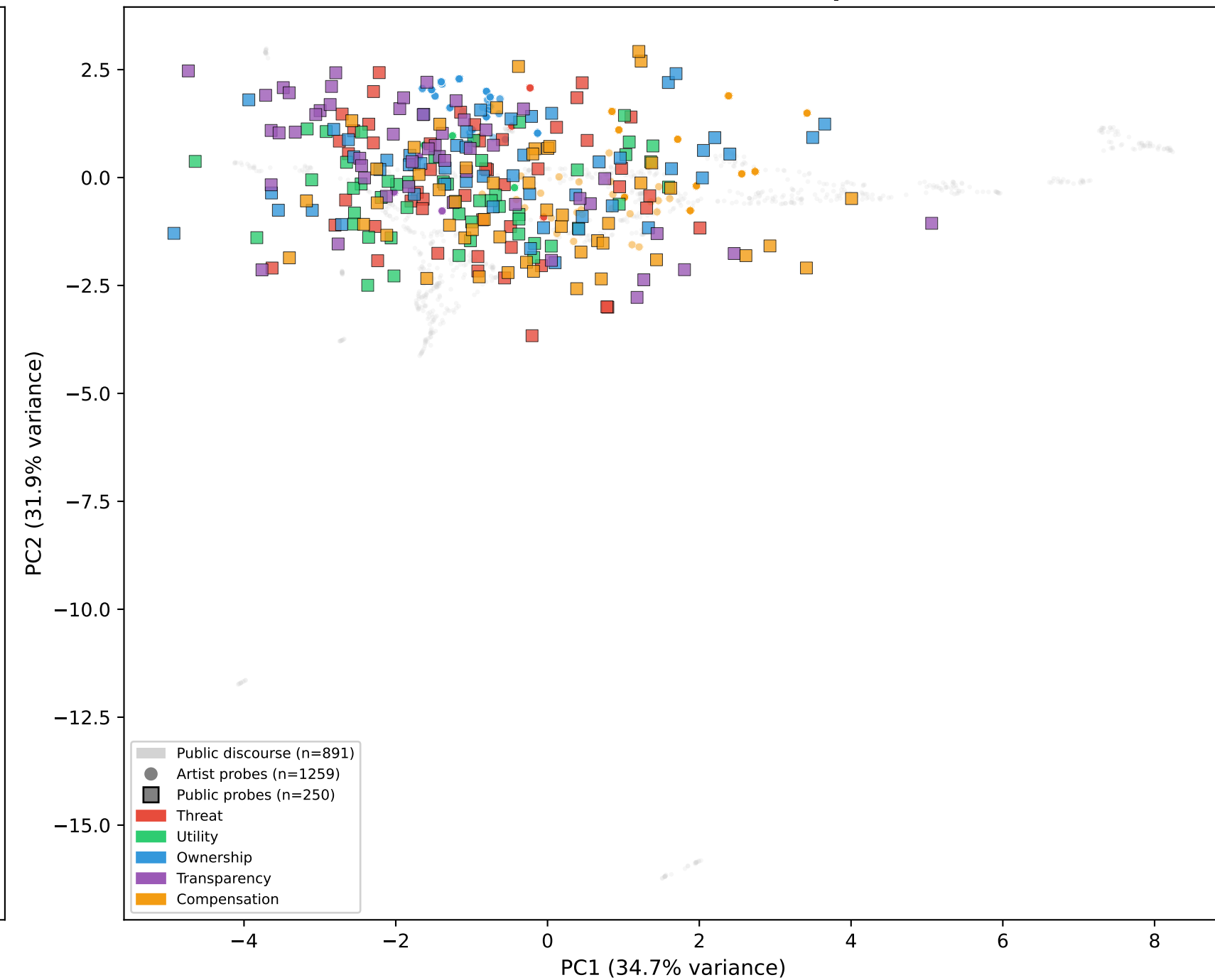
B. All Probes in Discourse Space
