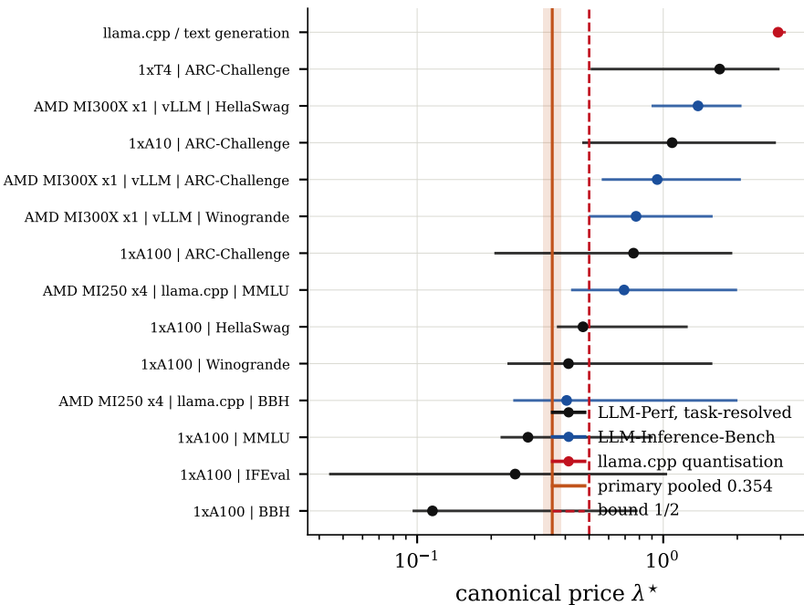
(a) 14 identified task-resolved LLM cells
