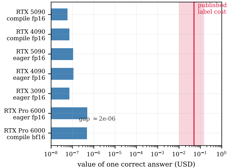
(b) v^* implied by \lambda^* vs. human labelling
