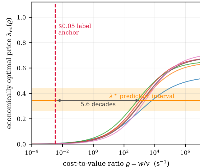
(a) The realised price is a bijection in \rho
