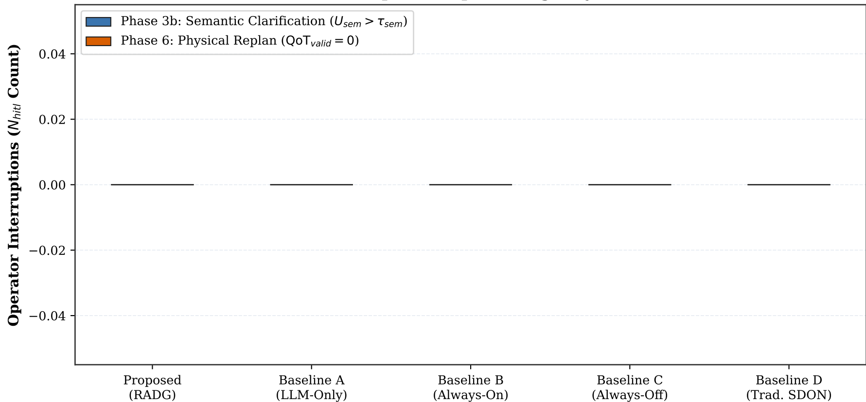
Human-in-the-Loop Interruption Origin by Decision Gate
