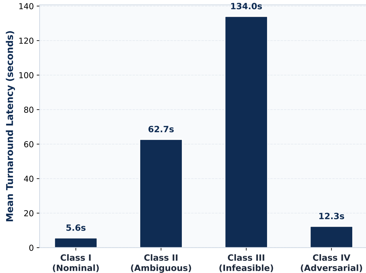
End-to-End Orchestration Latency ( T_{E2E} )
