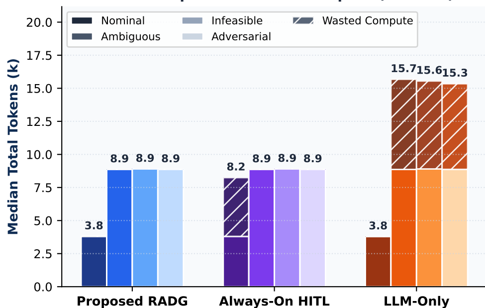
Token Footprint & Wasted Compute (kTokens)
