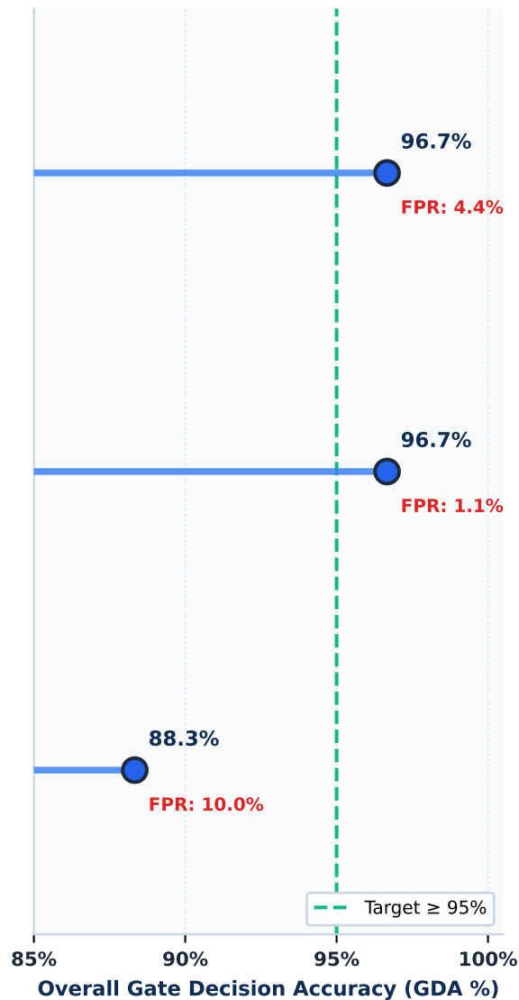
Overall GDA & FPR (Cleveland Scale)
