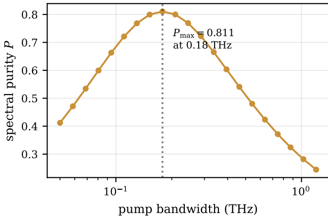
(a) bandwidth matching (ideal pump)
