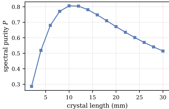
(b) length matching at 0.164 THz pump
