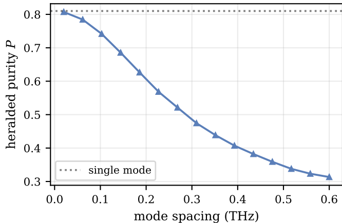
(b) spacing of a 3-mode comb
