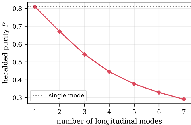
(a) modes at 0.25 THz spacing
