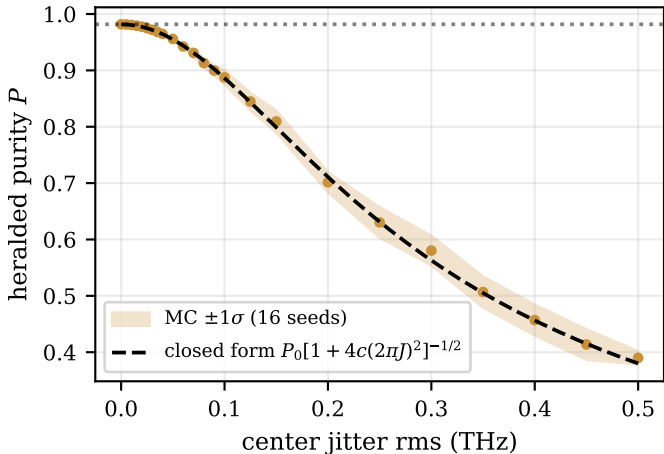
(a) Gaussian phase matching: exact benchmark
