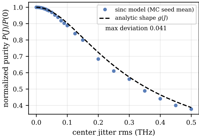
(b) sinc model: shape transfer
