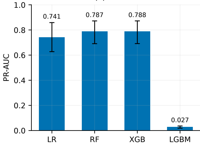
(a) PR-AUC
