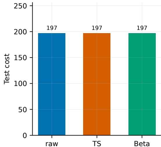
(a) XGB
