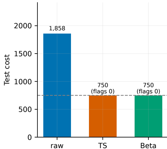
(b) LGBM (dashed: null-model cost 750)
