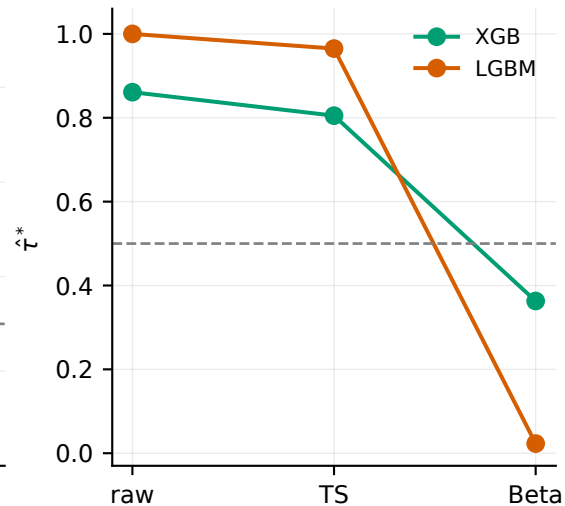
(c) frozen \hat{\tau}^* , XGB and LGBM, vs naive 0.5
