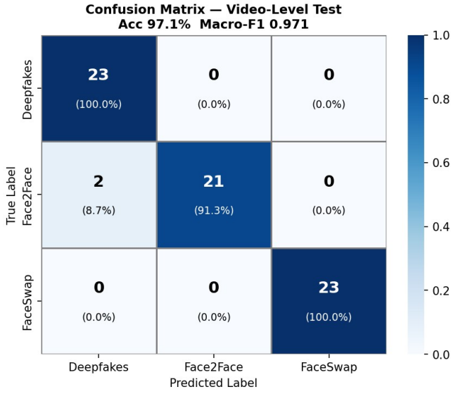
Fig. 9. Manipulation-type video-level (group) confusion matrix on the test set.
