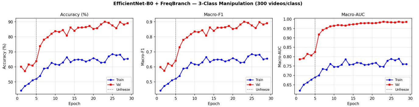
Fig. 7. Manipulation-type classifier training and validation curves (Accuracy, Macro-F1, ROC-AUC); the dashed line marks the backbone unfreeze point.
