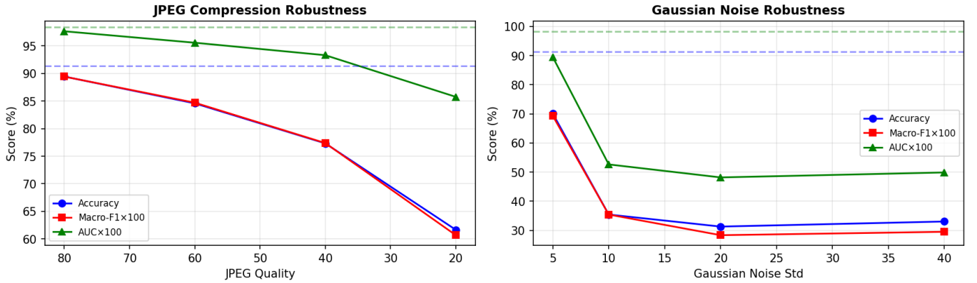
Fig. 12. Manipulation-type classifier robustness under JPEG recompression (left) and Gaussian noise (right).
