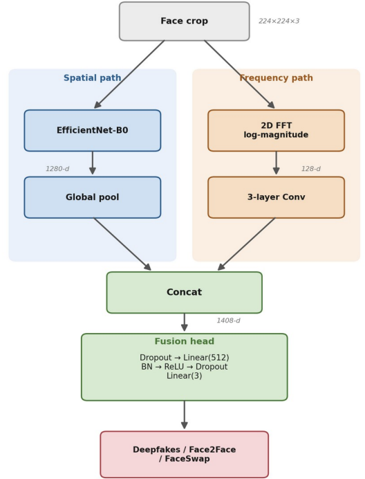
Fig. 1. Architecture of the dual-branch manipulation-type classifier: an EfficientNet-B0 spatial path and an FFT-based frequency path are concatenated and classified by a fusion head.
