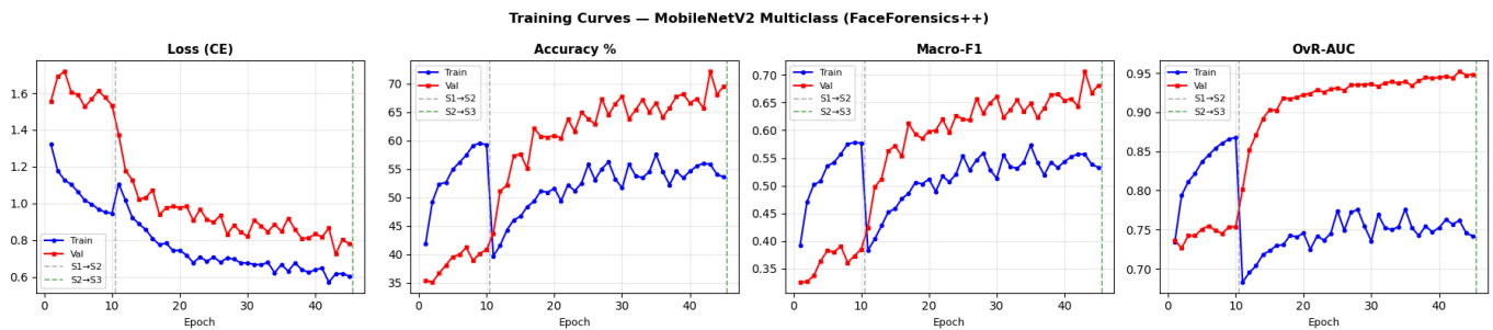
Fig. 16. Five-class model training and validation curves across the three fine-tuning stages.
