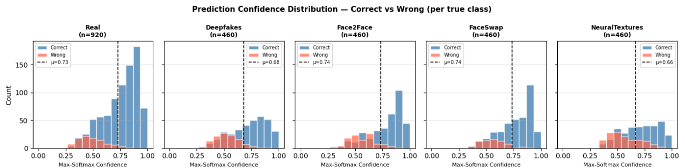
Fig. 18. Five-class prediction-confidence distributions, correct vs. wrong, per true class. Correct predictions cluster at high confidence; most errors fall below the per-class mean (dashed).
