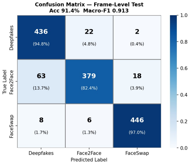
Fig. 8. Manipulation-type frame-level confusion matrix on the test set.
