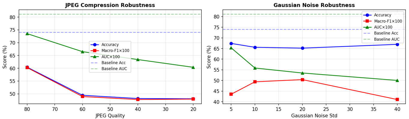
Fig. 6. Binary detector robustness under JPEG recompression (left) and Gaussian noise (right).
