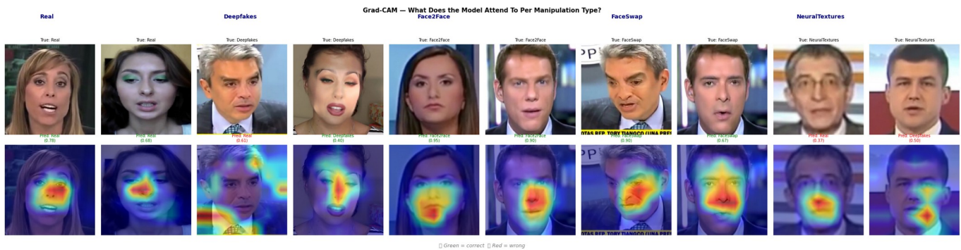
Fig. 17. Five-class model Grad-CAM overlays; attention concentrates on central facial regions for each class.
