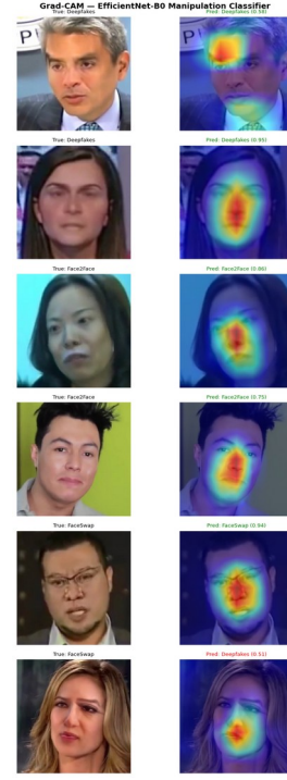
Fig. 11. Grad-CAM overlays for the manipulation-type classifier.
