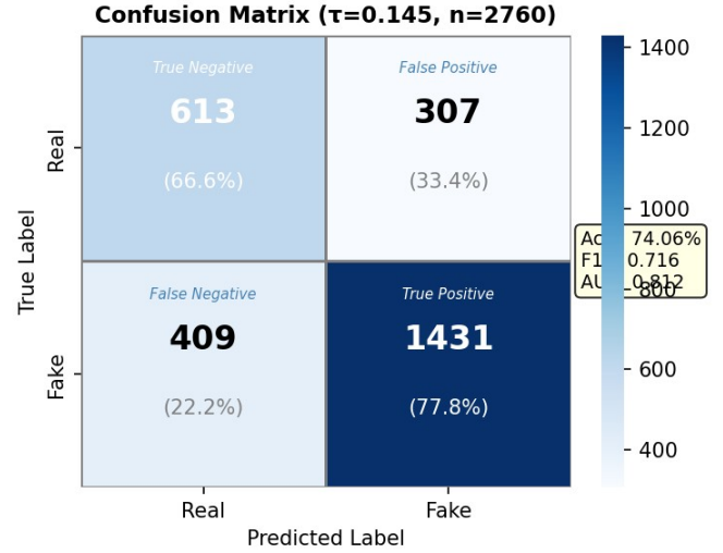
Fig. 3. Binary confusion matrix on the test set at the validation-tuned threshold; the real (minority) class is harder, with lower recall than fake.
