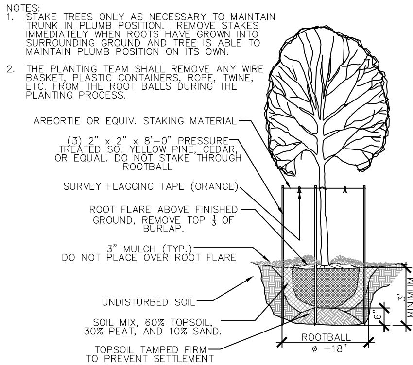
TYPICAL TREE PLANTING & STAKING N.T.S.
