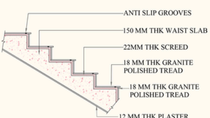
TYPICAL TREAD AND RISER DETAIL SCALE - 1:20
