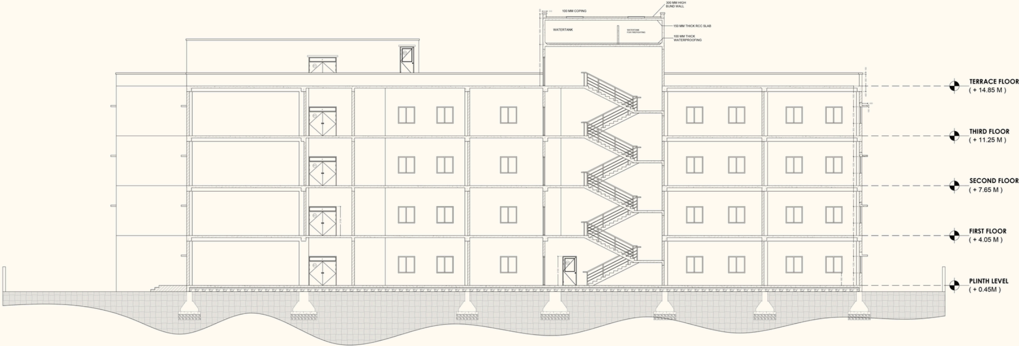
SECTION AA'
