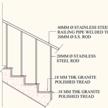
TYPICAL RAILING DETAIL SCALE - 1:20
