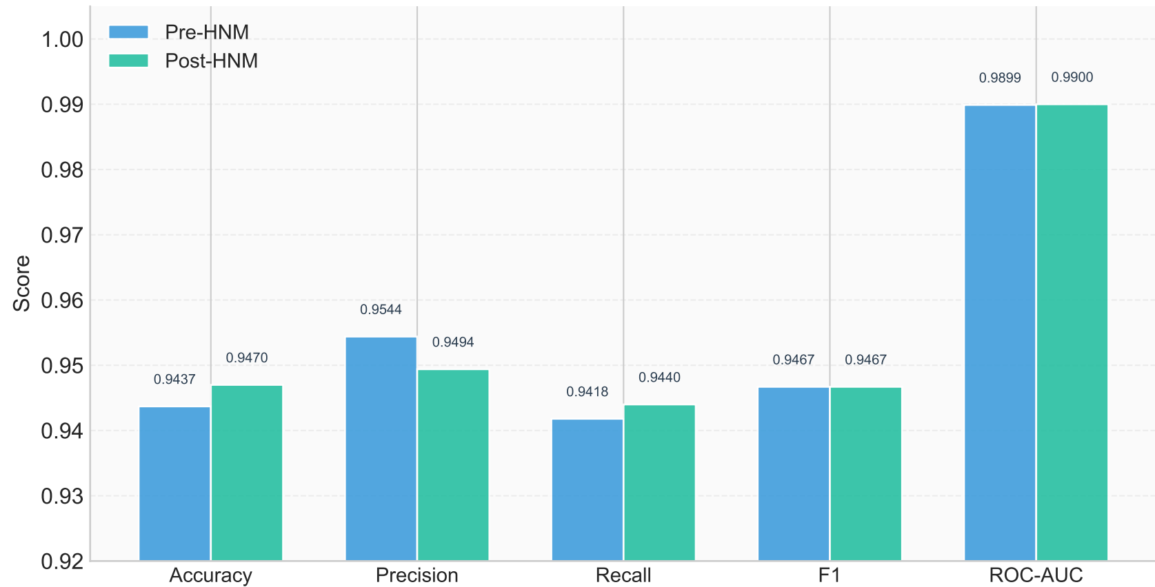
Pre-HNM vs Post-HNM Ensemble Performance (Frozen Test Set, N=3,980)
