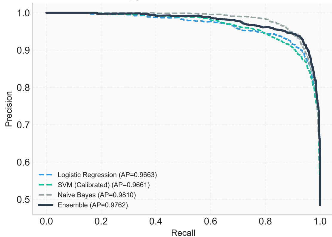
(b) Precision–Recall Curves
