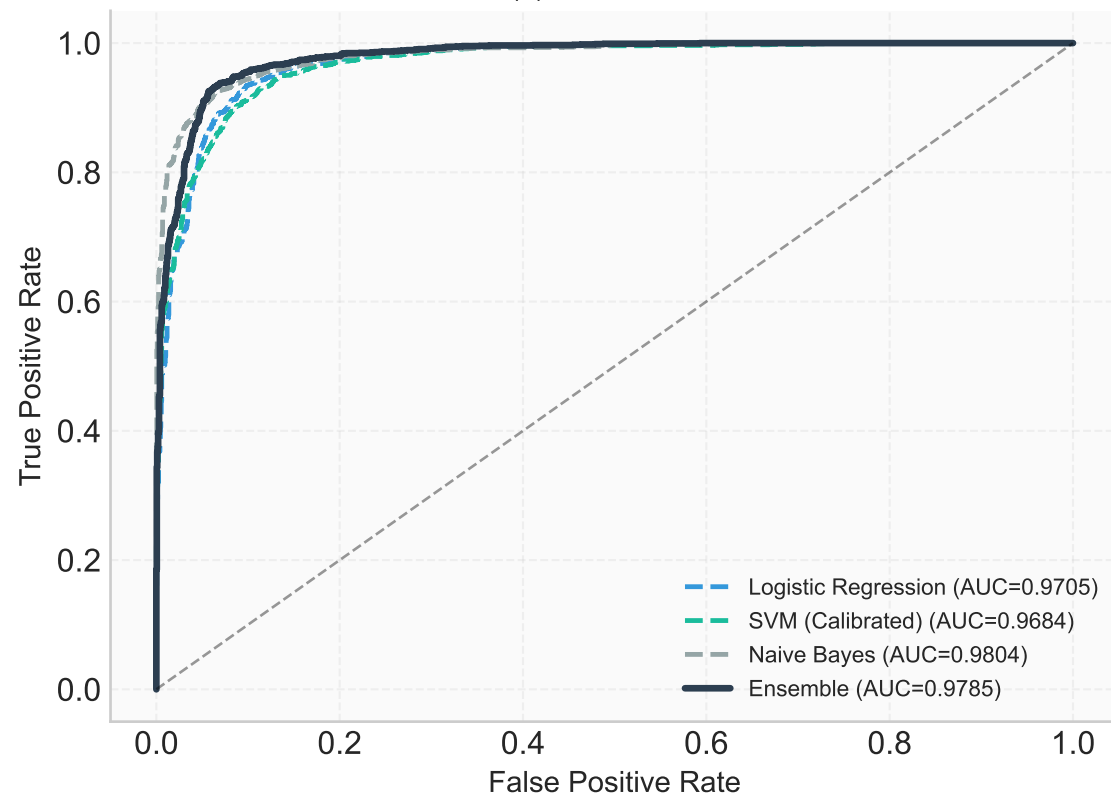
(a) ROC Curves
