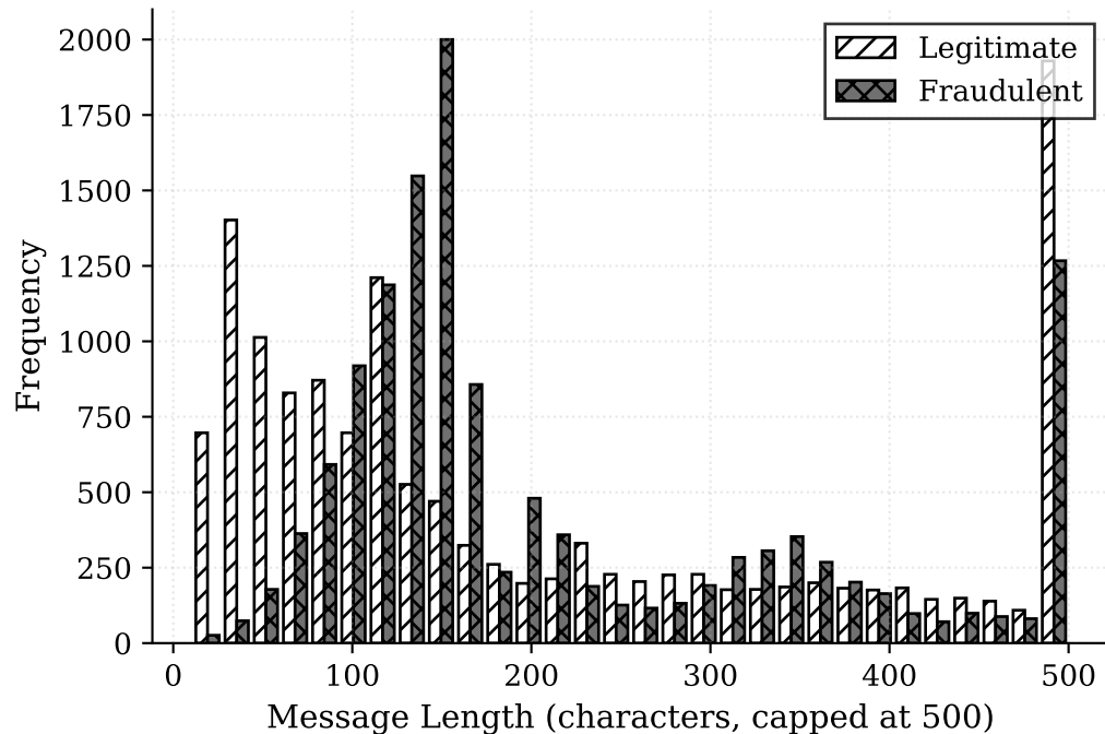
(b) Length Distribution by Class
