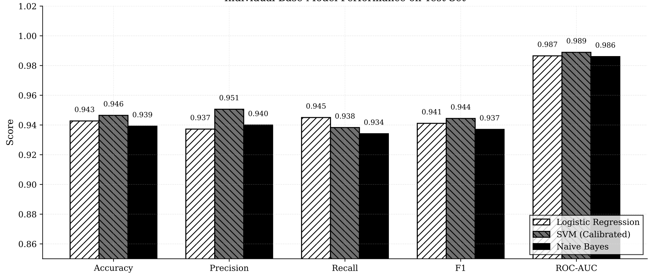
Individual Base Model Performance on Test Set
