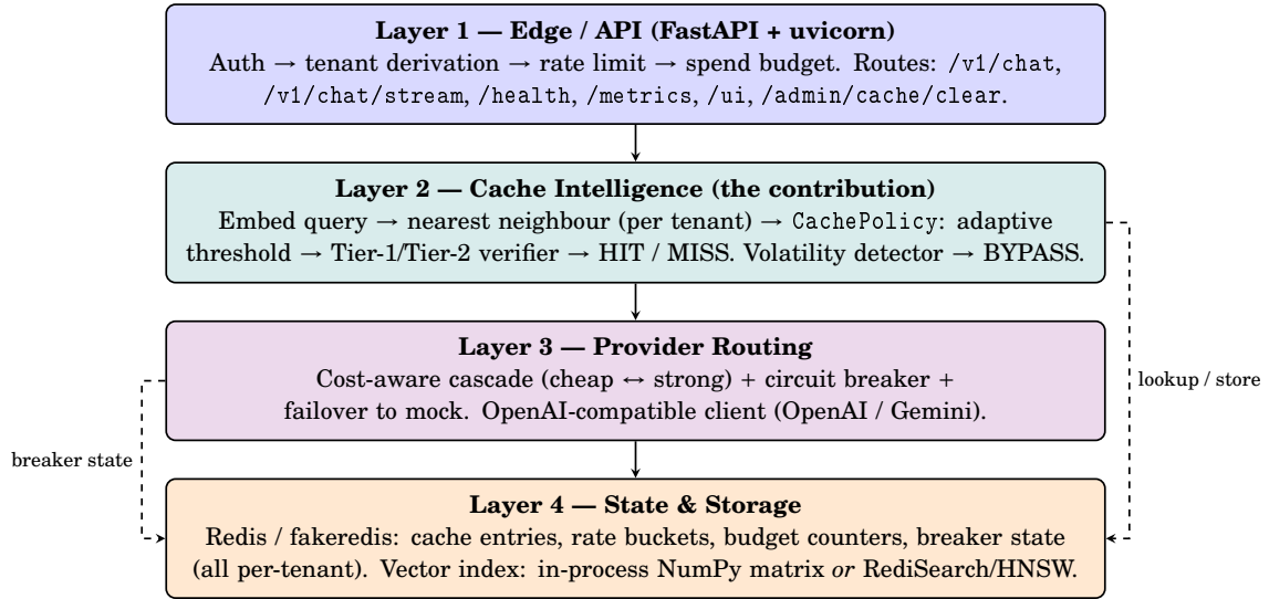
Figure 4.1: VeriGate four-layer architecture. Requests descend from the edge; a verified cache hit in Layer 2 short-circuits the provider call in Layer 3. All state in Layer 4 is namespaced per tenant.
