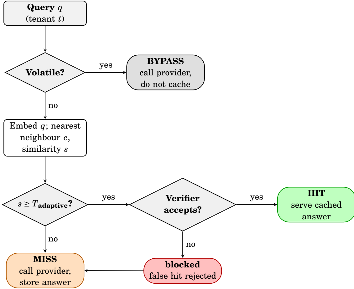
Figure 4.5: The four-outcome cache decision. A candidate whose similarity clears the adaptive threshold is still subjected to the verifier; only a verified candidate is served as a HIT, while a rejected one is demoted to a MISS (“blocked”). Volatile queries bypass the cache entirely.
