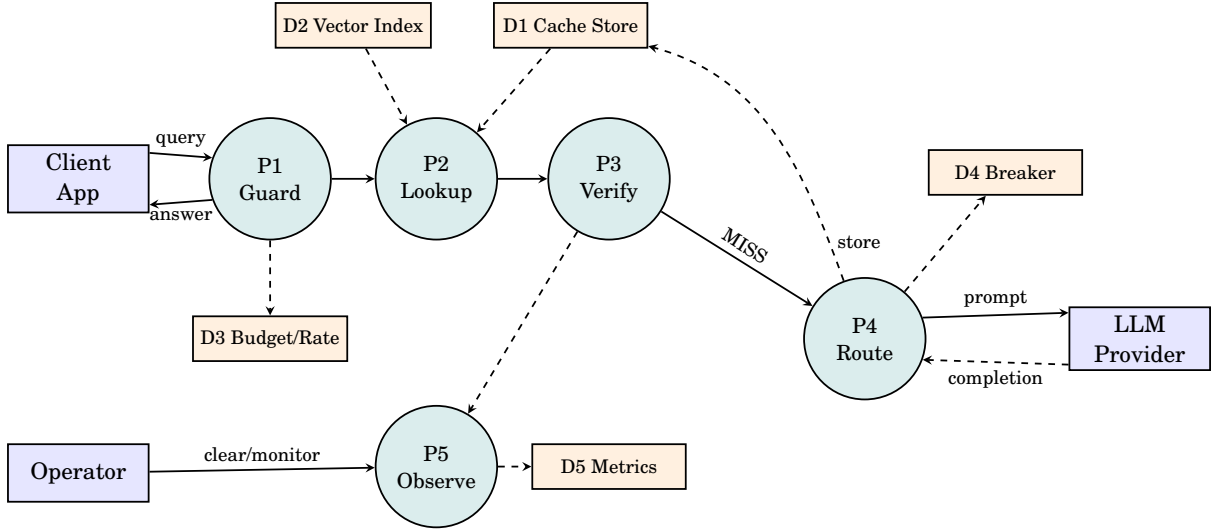
Figure 4.4: Level-1 DFD. Five processes (P1 Guard, P2 Lookup, P3 Verify, P4 Route, P5 Observe) operate over five data stores (D1 Cache, D2 Vector Index, D3 Budget/Rate, D4 Breaker, D5 Metrics). A verified hit in P3 answers the client directly; only a miss reaches P4 and the external provider.
