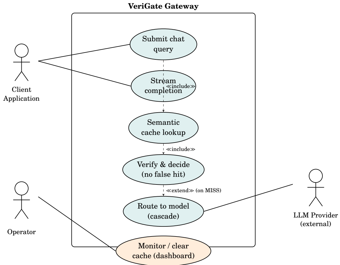
Figure 4.2: UML use-case diagram. The Client Application submits and streams queries; every submission includes a cache lookup and a verify-and-decide step, and extends to a model route only on a miss. The Operator monitors and clears the cache; the external LLM Provider fulfils missed calls.
