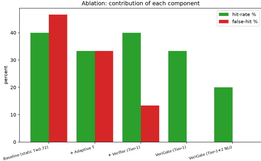
Figure 6.2: Ablation bars: hit-rate (green) and false-hit rate (red) as components are added. False-hit rate falls step-by-step to zero for full VeriGate while hit-rate stays reasonable.
