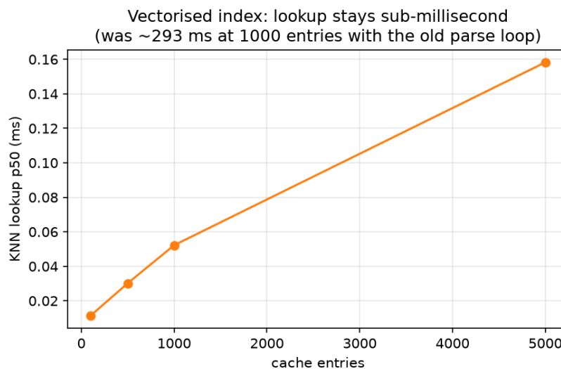
Figure 6.4: KNN lookup latency versus cache size. The vectorised in-process index stays sub-millisecond and near-flat to 5000 entries, versus ~293 ms at 1000 for the original parse loop.
