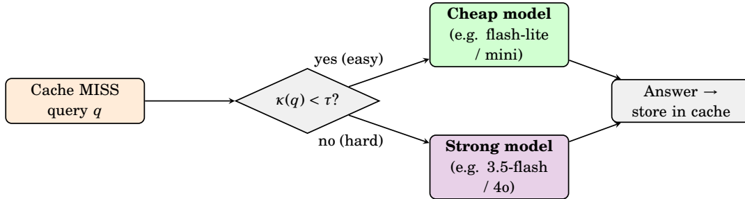
Figure 4.3: Cost-aware cascade. A transparent complexity score routes easy queries to the cheap model and escalates only hard ones to the strong model; the unused tier remains as a failover.
