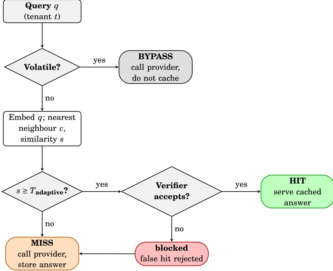
Figure 4.2: The four-outcome cache decision. A candidate whose similarity clears the adaptive threshold is still subjected to the verifier; only a verified candidate is served as a HIT, while a rejected one is demoted to a MISS (“blocked”). Volatile queries bypass the cache entirely.
