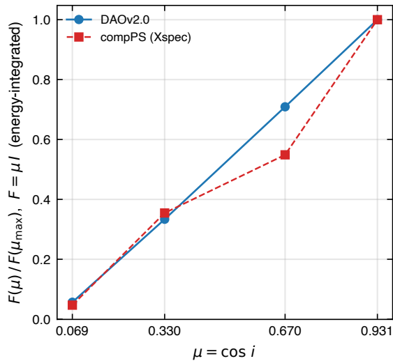
Limb-darkening law
