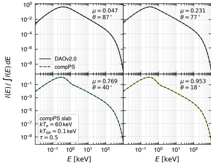
Flux-normalised emergent spectra
