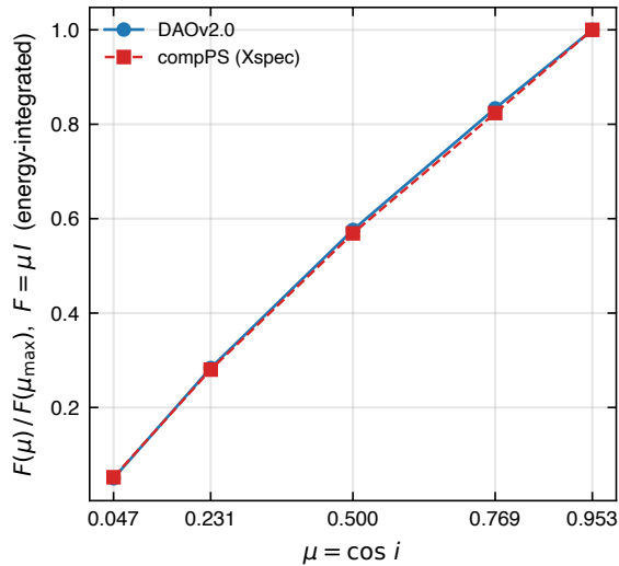
Limb-darkening law
