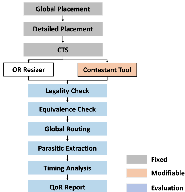
Figure 1. ISPD 2027 Contest flow. The contestant's buffering and sizing tool replaces the OpenROAD Resizer step. Fixed placement and CTS stages (gray) provide inputs; the evaluation flow (blue) performs equivalence checking, global routing, parasitic extraction and timing analysis to measure QoR.
