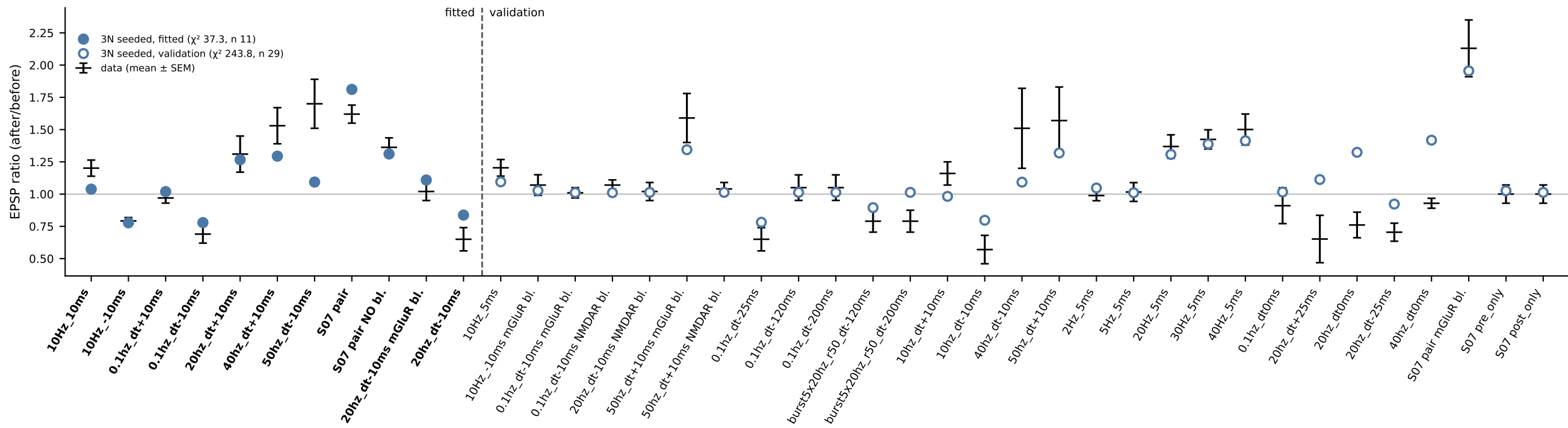
(A) L5→L5: 11 fitted, 29 validation
