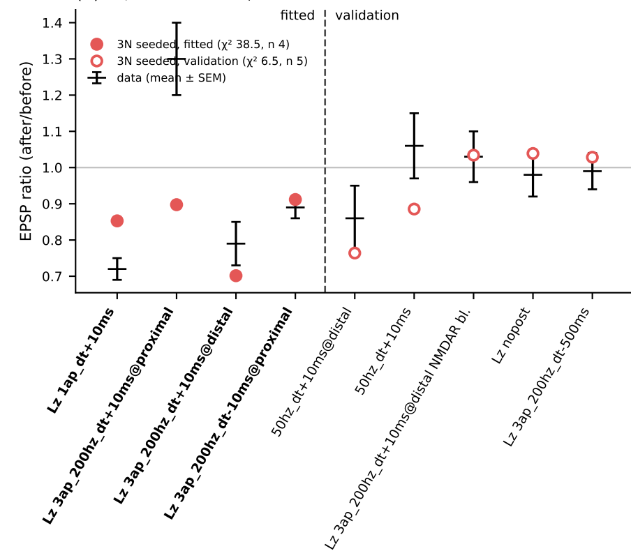
(B) L2/3→L5: 4 fitted, 5 validation
