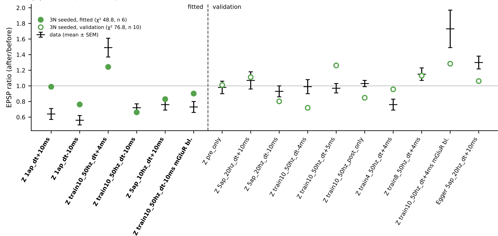
(C) L2/3→L2/3: 6 fitted, 10 validation
