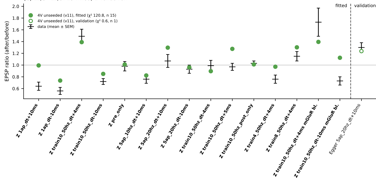
(C) L2/3→L2/3: 15 fitted, 1 validation
