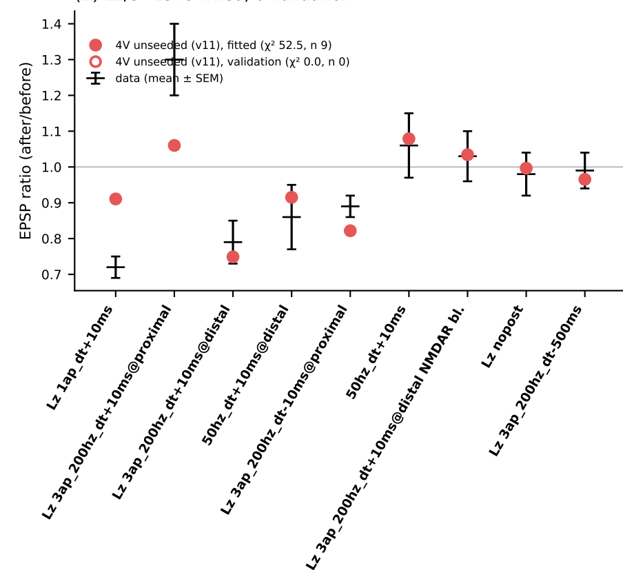
(B) L2/3→L5: 9 fitted, 0 validation
