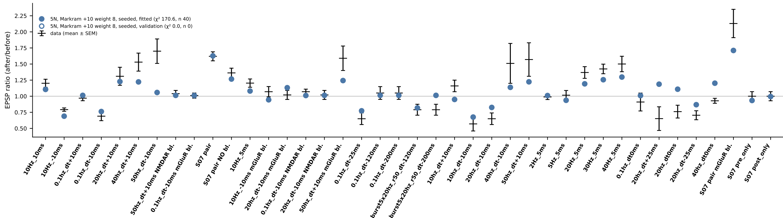
(A) L5→L5: 40 fitted, 0 validation
