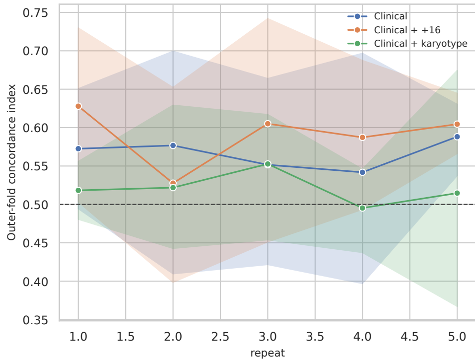
Repeated nested-CV survival models
