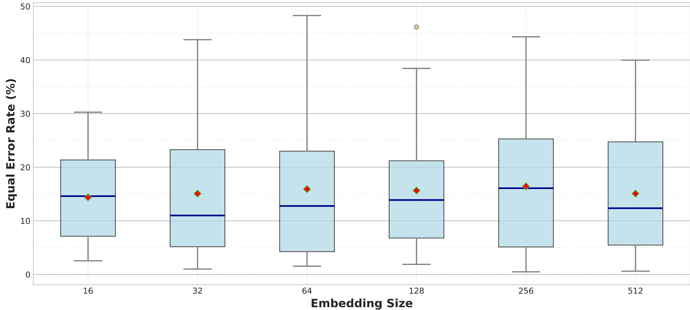
Distribution of Equal Error Rate by Embedding Size
