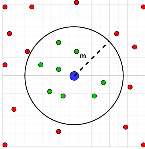
Figure 2.3: Figure demonstrating the effect of the margin hyperparameter m on the contrastive loss function. The model optimizes the feature representations so every element within radius m around certain reference shares the same class, while the elements outside this area have different classes.
