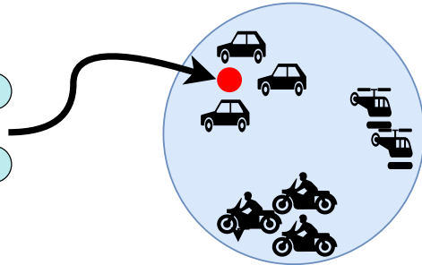
Feature Space
