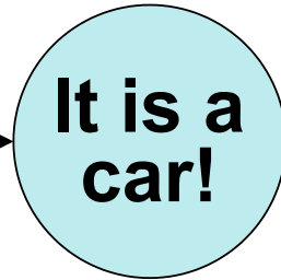
Classification
