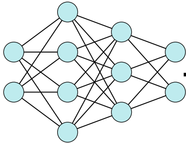
Neural Network
