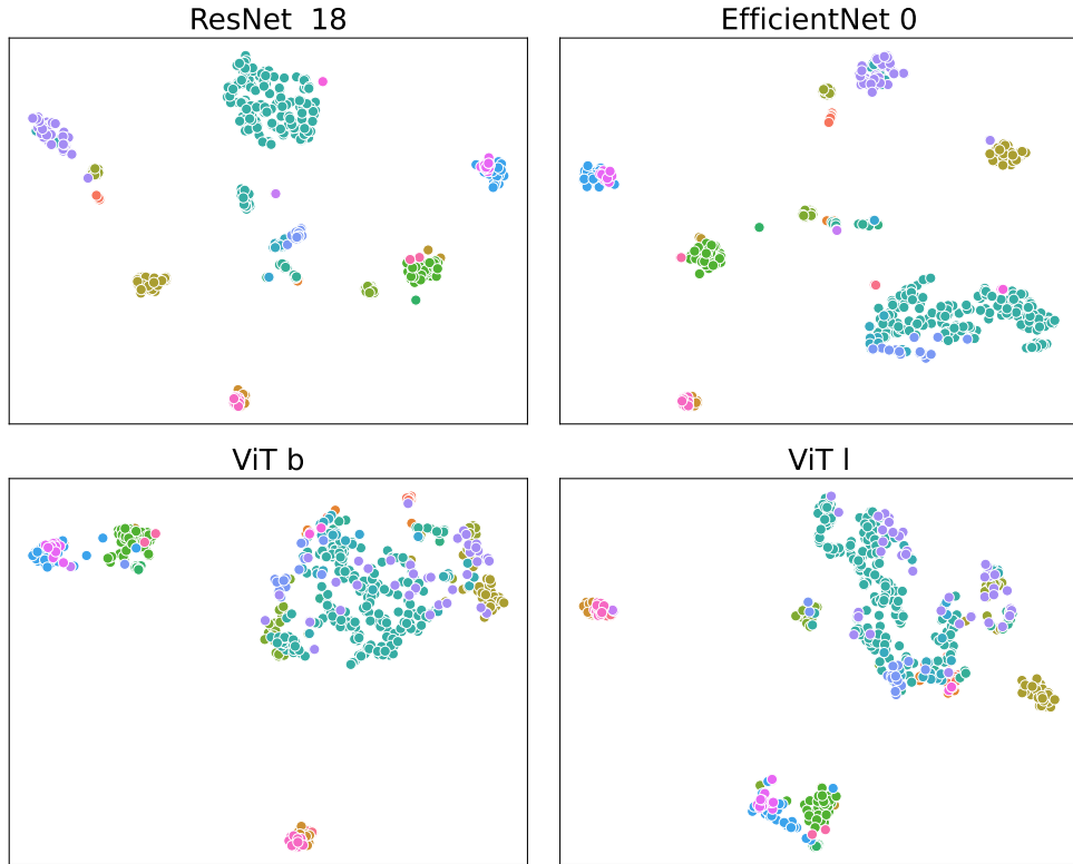
Figure 5.2: TSNE visualization of the Test ZSL scenario. These models were trained on the same cross-validation fold. Each dot represents a document positioned in this two-dimensional space through TSNE dimensionality reduction. Each color represents a different class.
