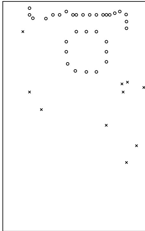
Drill Map: x 0.300mm / 0.0118" (11 holes) o 0.400mm / 0.0157" (32 holes)
