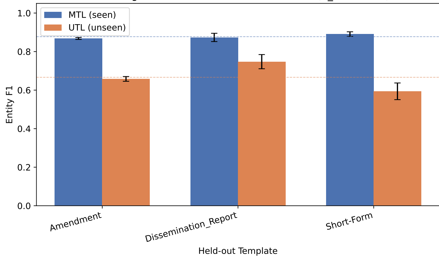
VRDU Registration Forms · LiLT · MTL vs UTL (n_train=200)
