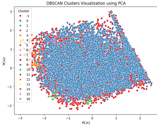
Fig. 2: DBSCAN clustering visualization using PCA.
